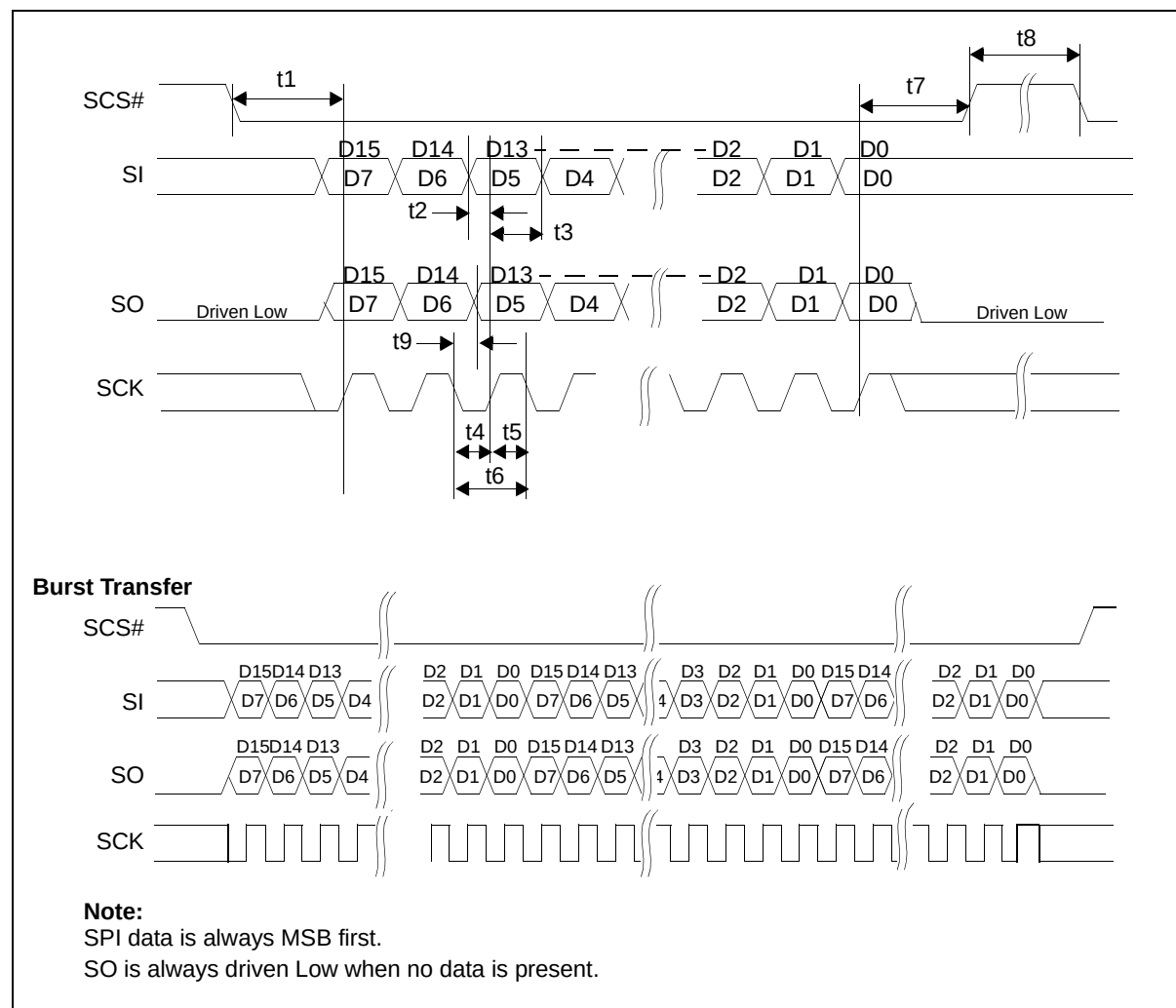
Figure 9-12: SPI Timing
