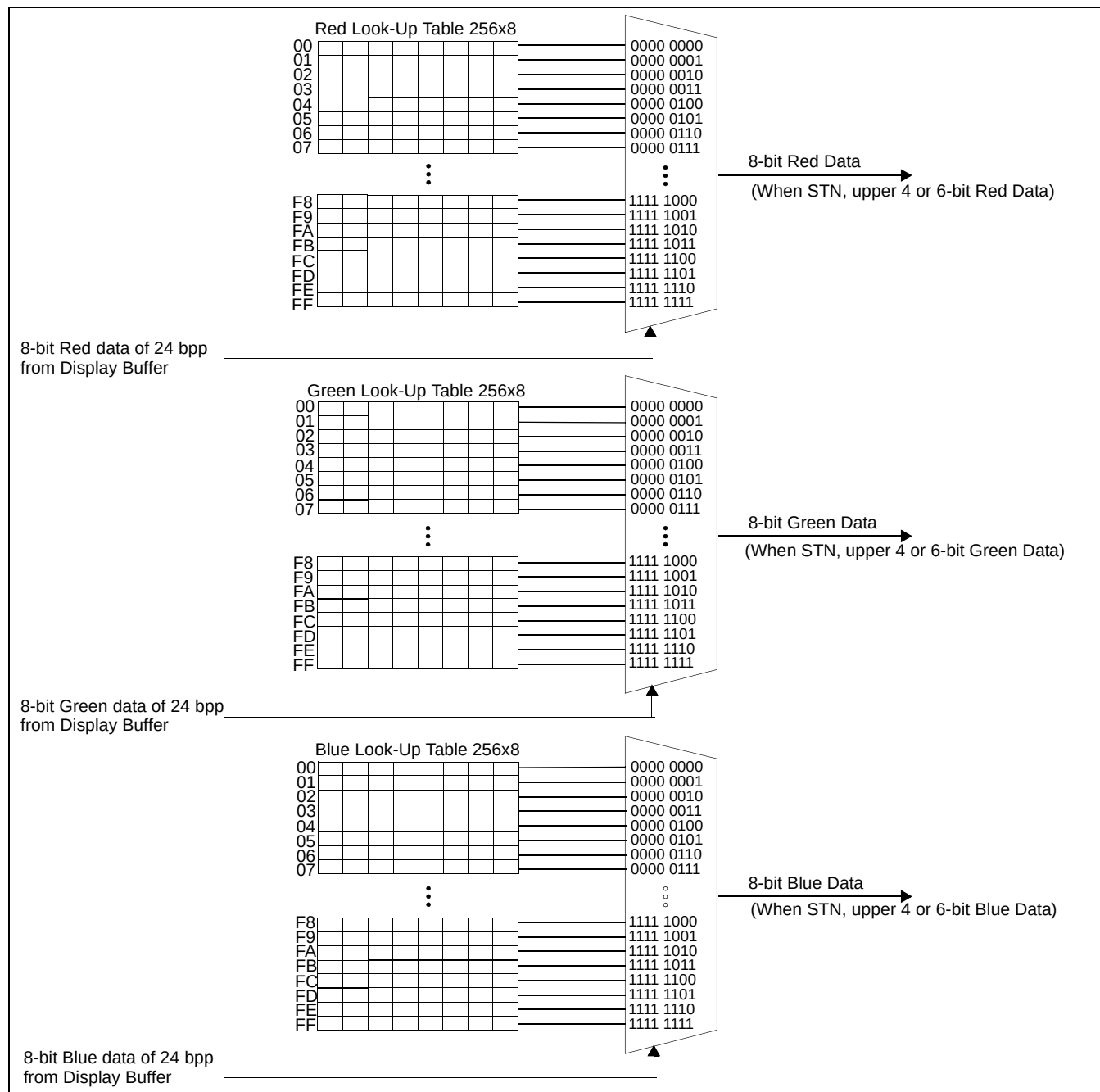
Figure 13-1: 24 bpp LUT
