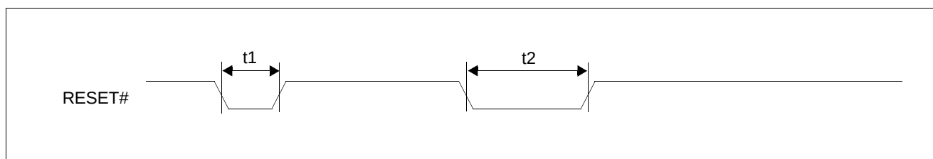
Figure 9-3 RESET# Timing
