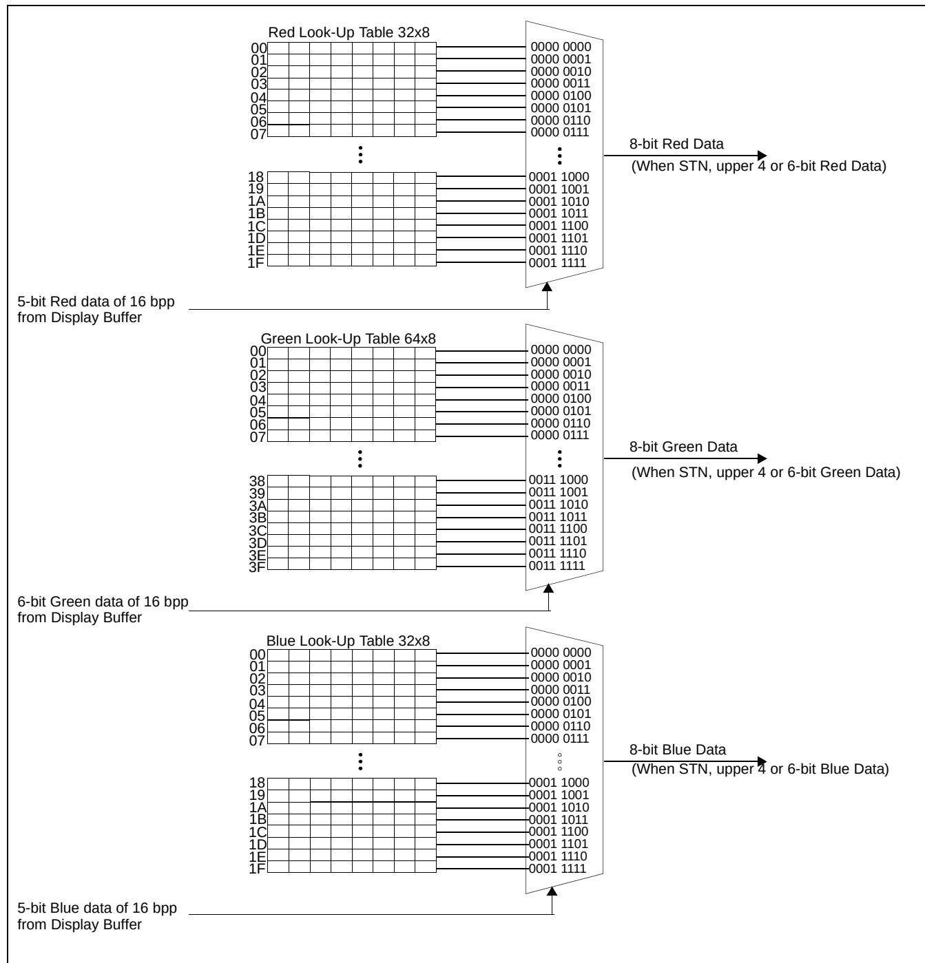
Figure 13-2: 16 bpp LUT
