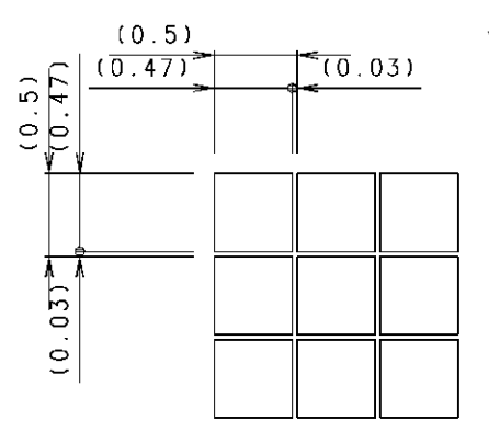
DOT DETAIL (S=20:1)
